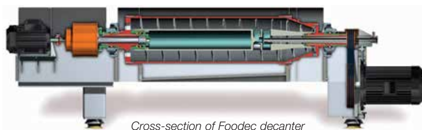
Cross-section of Foodec decanter
